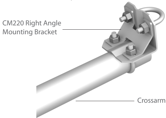
A closeup of the CM220 Right Angle Mounting Bracket shows the construction and crossarm attachment.
