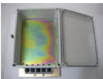
weatherproof enclosure @ L:38cm W:28cm H:18cm
