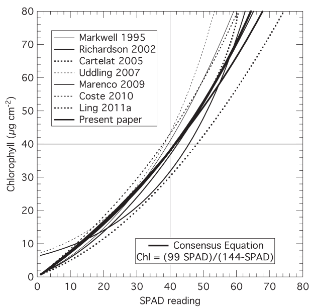
Fig. 4. Comparison of the calibration models for SPAD-502 available in the literature. All data were adjusted to common units for Chl in \mu\text{g cm}^{-2} . The functions for the eight models plotted on the graph from which the consensus equation was derived were: y = 0.09 10^{(x \wedge 0.265)} (Markwell et al. 1995); y = 0.552 + 0.404x + 0.0125 x^2 (Richardson et al. 2002); y = 93.6 - 11.9 \sqrt{(62 - x)} (Cartelat et al. 2005); y = 6.91 e^{(0.0459x)} (Uddling et al. 2007); y = 6.205 e^{(0.0408x)} (Marengo et al. 2009); y = (117.1x)/(148.84 - x) (Coste et al. 2010) y = 0.9 (0.381 + 0.4119x + 0.0105x^2) (Ling et al. 2011a, 2011b); y = (138x)/(185 - x) (present paper).
