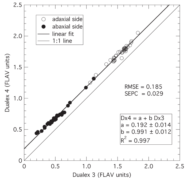
Fig. 2. Comparison of the flavonoid meter function of Dualex 4 Scientific to the Dualex 3. Adaxial and abaxial sides of grapevine leaves were measured with the two devices, and a linear model was fitted. RMSE and SEPC are indicated in the graph along with the coefficient values of the model with their \pm 95\% confidence intervals.
