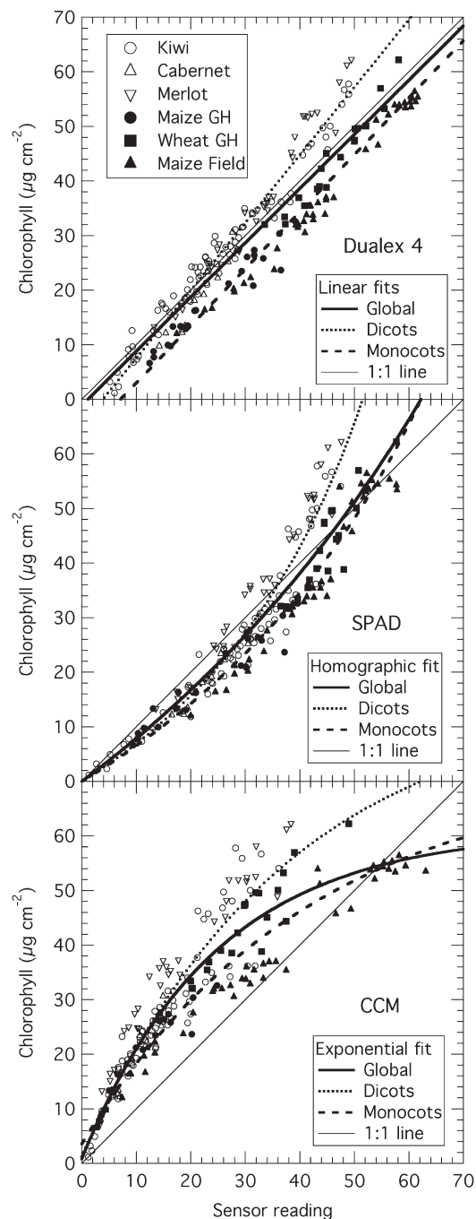
Fig. 3. Calibration of the three sensors against the chlorophyll extracts. Dicot plants are indicated with open symbols and monocots with closed symbols. All dicot leaves came from the field and monocot leaves were either from greenhouse (GH) grown plants or from the field. Fits for global models encompassing all data points are plotted along with the fits for the dicot and monocot plants independently: for Dualex linear ( a + bx ), for SPAD homographic ( (ax)/(b-x) ) and for CCM exponential ( a + be^{\alpha x} ); P < 0.0001 for all models. Coefficients of the models are presented in Table 2.
